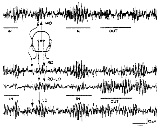
FIGURE 3. A comparison of referential and bipolar EEG recordings from right and left occipital lobes when brainwave activity is in phase and out of phase. (RO = right occipital; LO = left occipital; MO=mid occipital).
