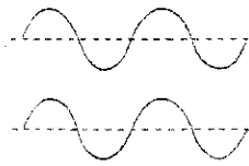
FIGURE 1. Two waves shown in-phase
